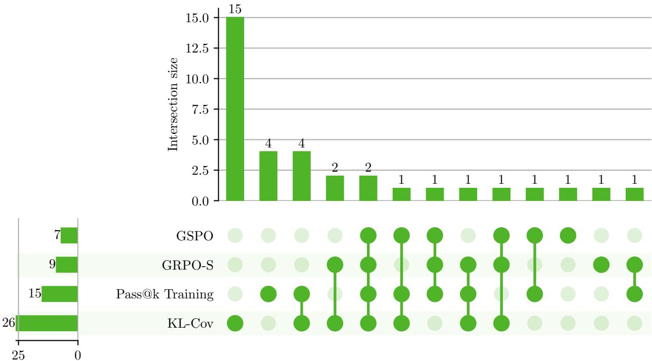
Expansion Intersections (pass@256 Base=0, RL=1), Model: Llama3.1-8B-Instruct
